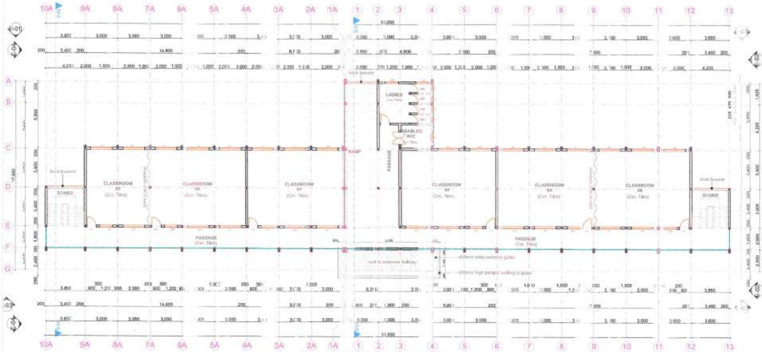
FIRST FLOOR FLOOR PLAN, SCALE 1:100
