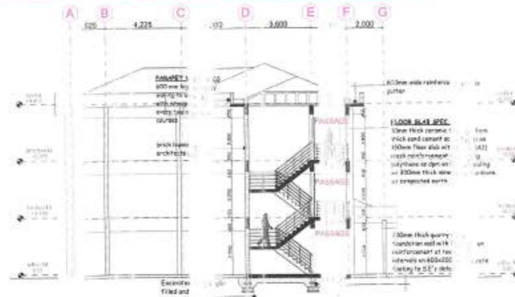
SECTION S-02, SCALE 1:100
