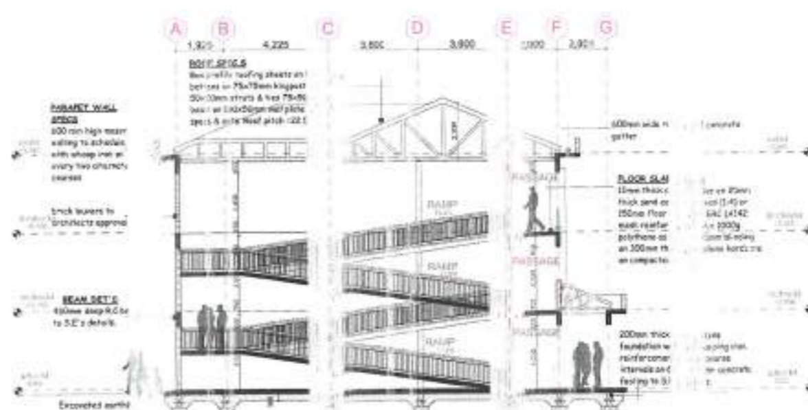
SECTION S-01, SCALE 1:100
