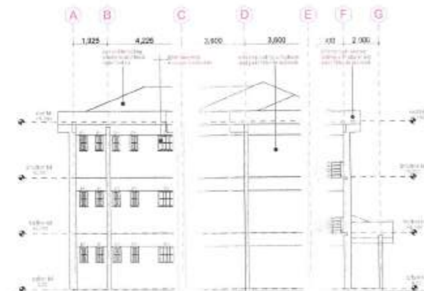
ELEVATION E-04, SCALE 1:100
